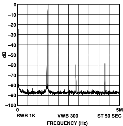
TPC 10. f_{MCLK} = 10 MHz, f_{OUT} = 1.43 MHz = f_{MCLK}/7 , Frequency Word = 2492492
